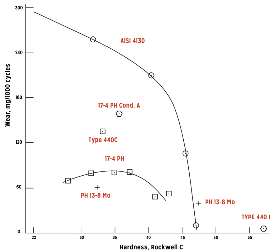
FIGURE 1 Effect of Hardness on the Wear of Heat Treatable Steels
